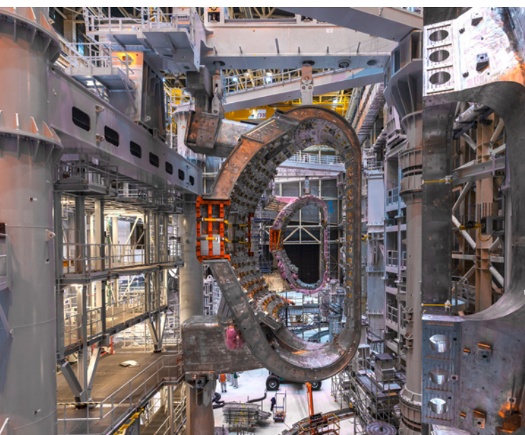
Vacuum vessel sectors at ITER
