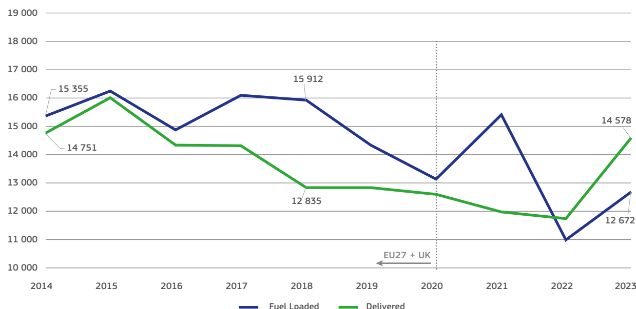
Figure 3. Natural uranium equivalent feed contained in fuel loaded into EU reactors and natural uranium equivalent delivered to utilities under purchasing contracts (tonnes NatU)
