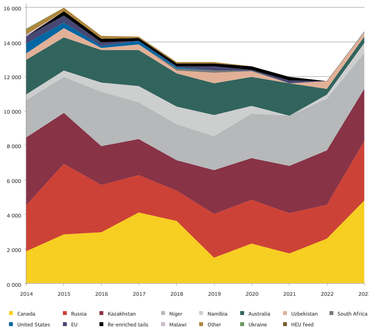
Figure 6. Purchases of natural uranium by EU utilities, by origin, 2014-2023 (tU)
