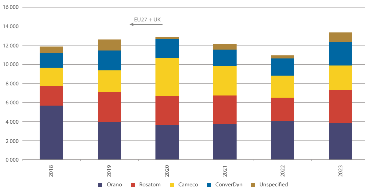
Figure 7. Supply of conversion services to EU utilities by provider, 2018-2023 (tU)
